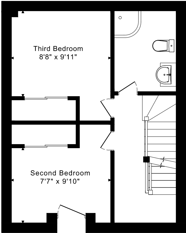
THIRD FLOOR 429 SQUARE FEET
