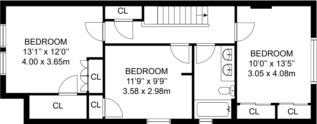
2ND LEVEL
