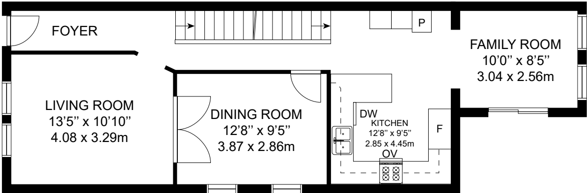
MAIN LEVEL
