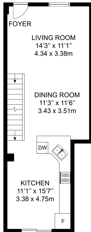
MAIN LEVEL
