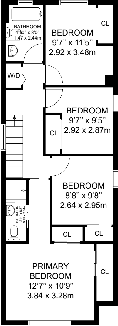
2ND LEVEL
