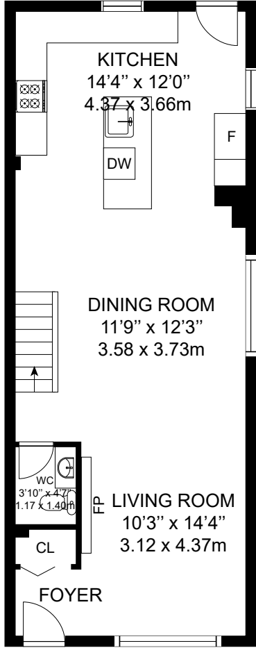
MAIN LEVEL
