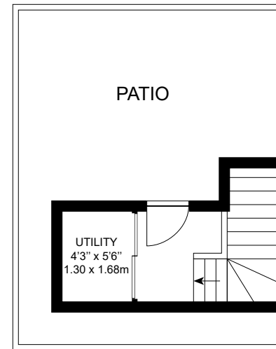
4TH LEVEL
