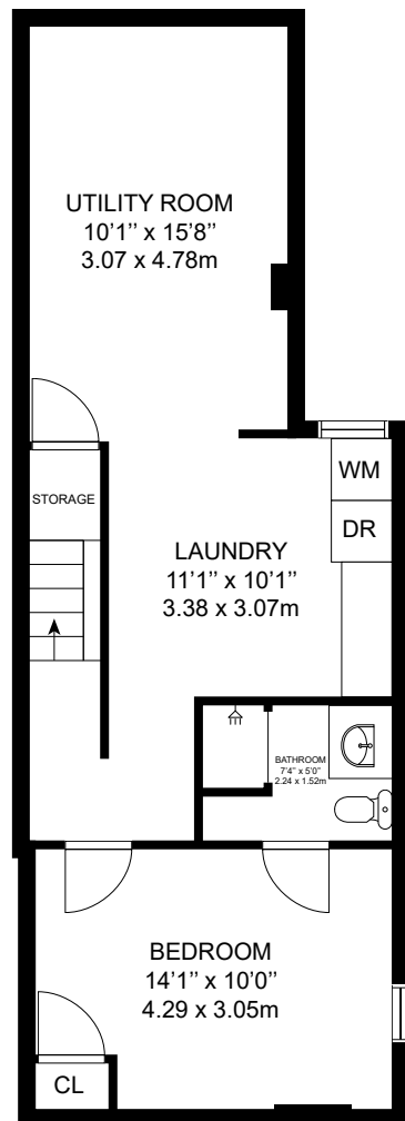
LOWER LEVEL
